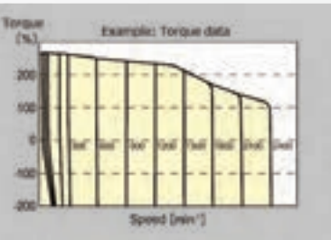
When a Toshiba standard 3-phase 400V-1.5kW motor is driven by the VFS15-4015PL-W1 after parameters are set.
