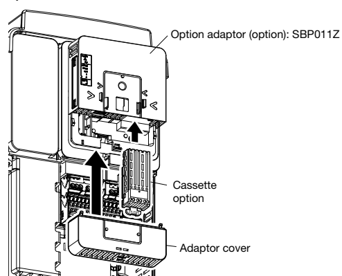
Option Slot C
