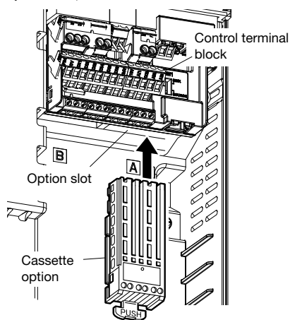
Option slot A, B
